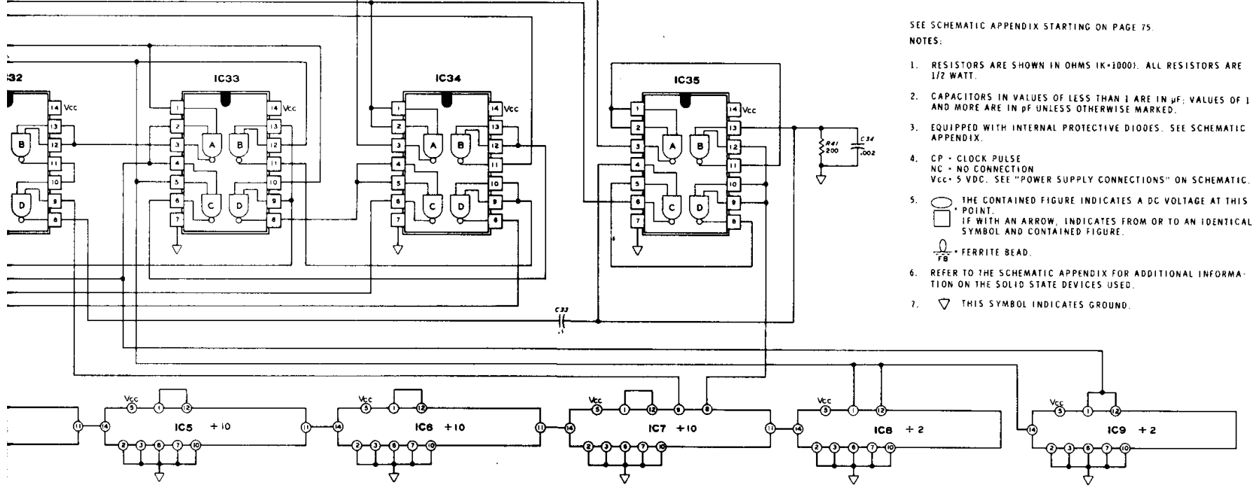
SCHEMATIC OF THE HEATHKIT® DIGITAL FREQUENCY DISPLAY MODEL SB-650
